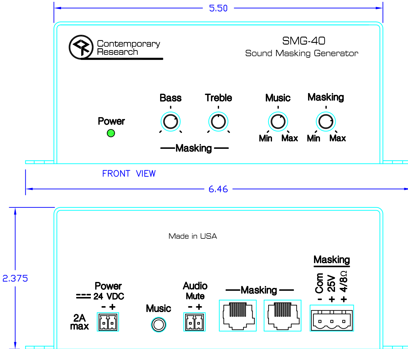
REAR VIEW
